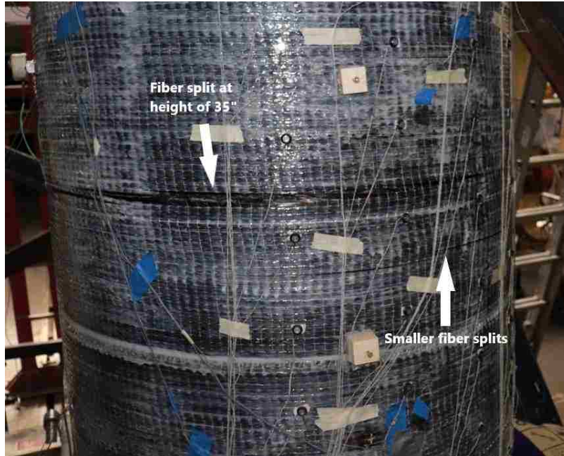
Figure 7-10. Fiber splitting on north face during Series 10
