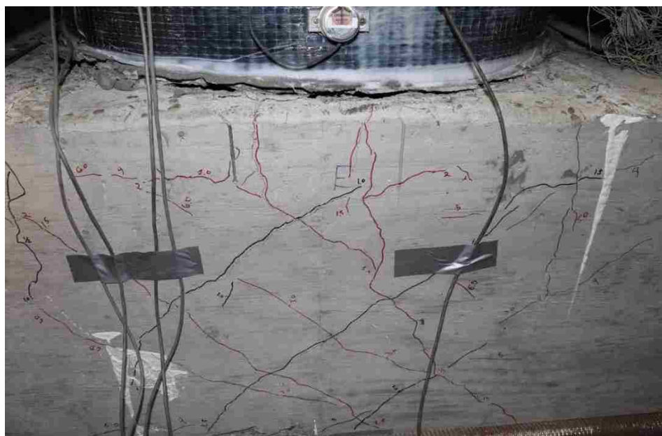
Figure 7-5. Progressive joint shear cracking on base beam on Series 8 (+4.70%, -5.49% drift)
