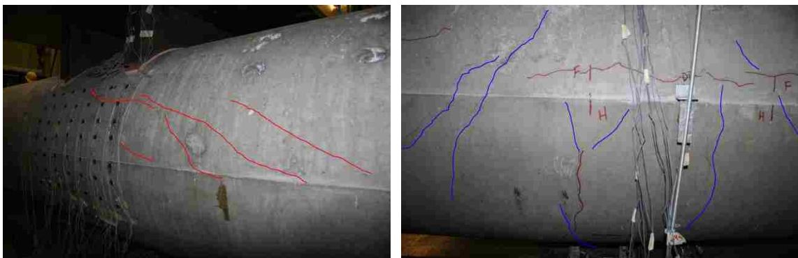
Figure 4-1. Progression of cracks on the west (left) and east (right) faces of specimen
