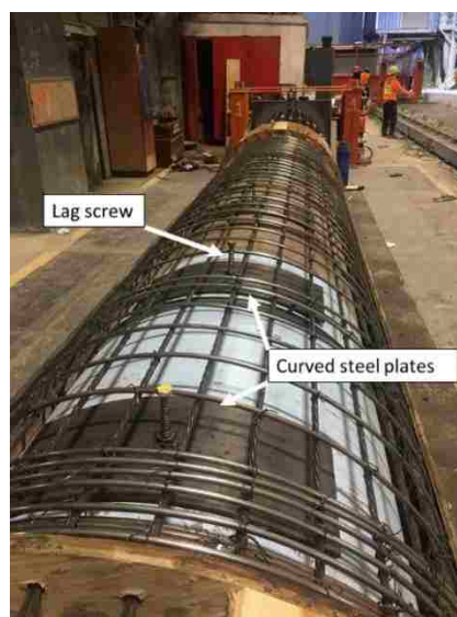
Figure 3-11. Hold-down plates used for sonotube during casting
