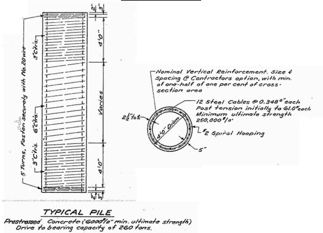
Figure A-1. Details of hollow prestressed concrete pile-column (Ravenna)
