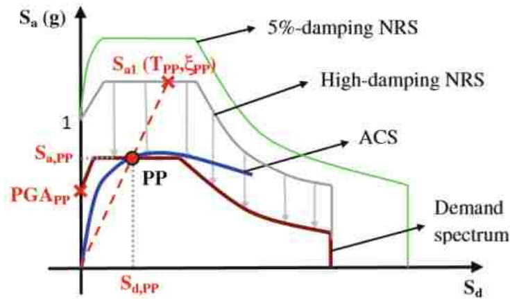
Figure 9-2. Acceleration-Displacement Response Spectrum (Cardone et. al, 2011)
