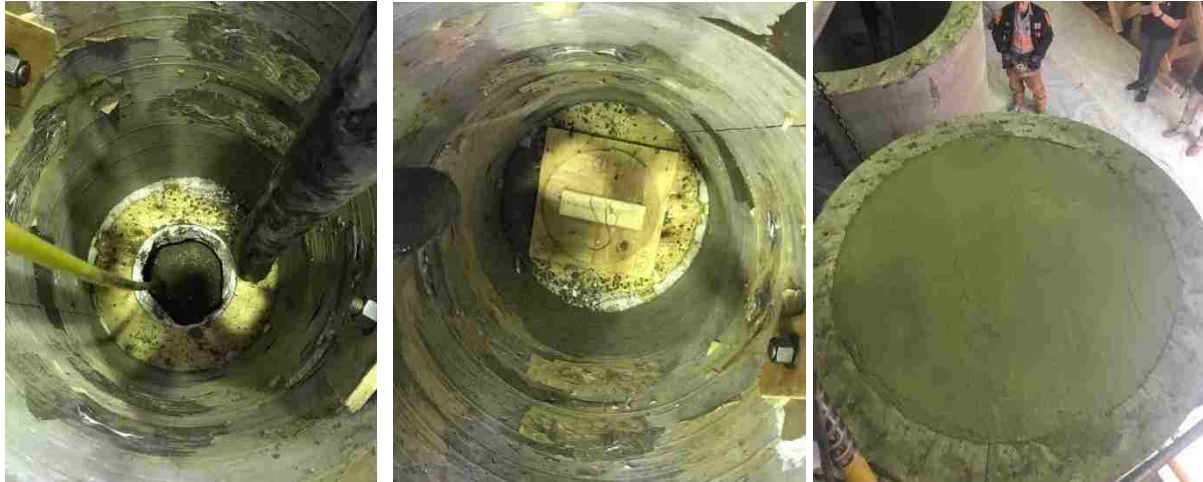
Figure 3-17. Left: Bottom half of fill concrete; Middle: Wood plug inserted; Right: Top half of fill concrete
