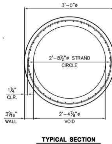
Figure 3-3. Cross-section view of test pile-column, showing dimensions (courtesy of Concrete Technology Corporation)
